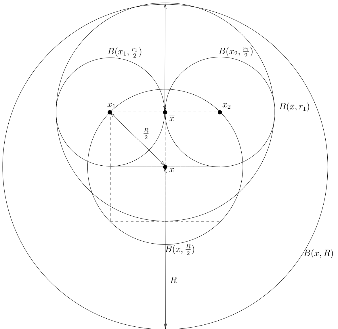
Figure 3.1: The diagram shows a case when B(\bar{x}, r_1) is not quite contained in B(x, R) .
