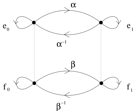
Figure 1.4.5: groupoid \mathbb{I} .
