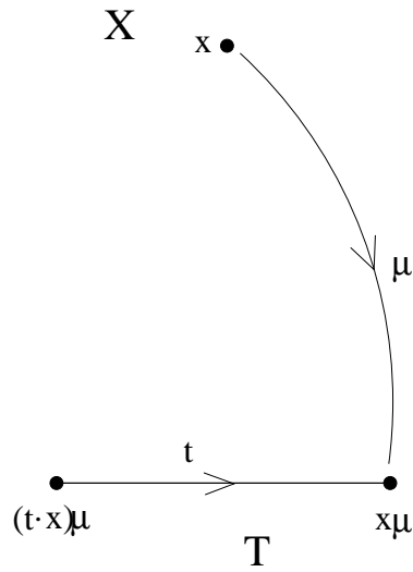
Figure 5.3.2: axiom (2).
