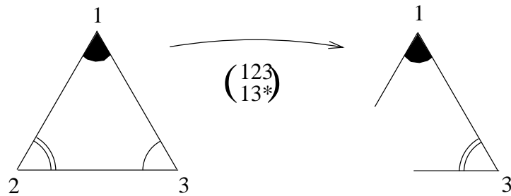
Figure 1.1.2: partial bijection.
