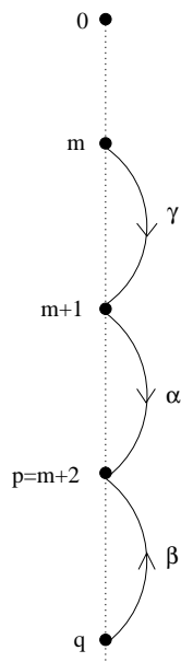
Figure 2.2.3: restriction
