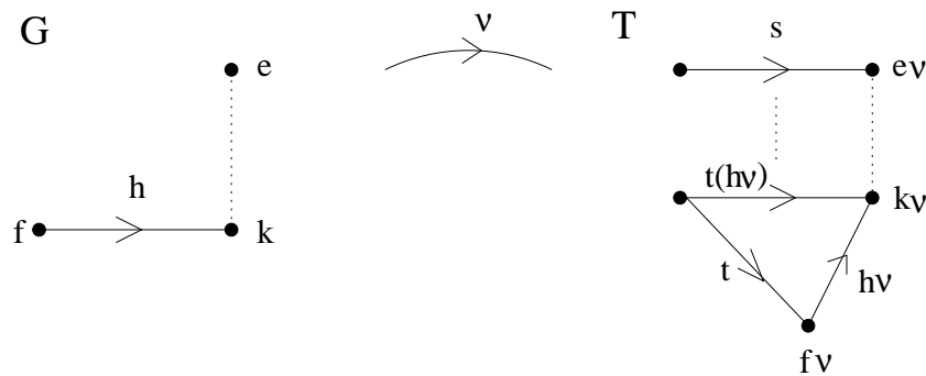
Figure 5.4.1: ordering.
