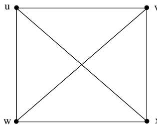
Figure 1.2.2: isomorphic graph.
