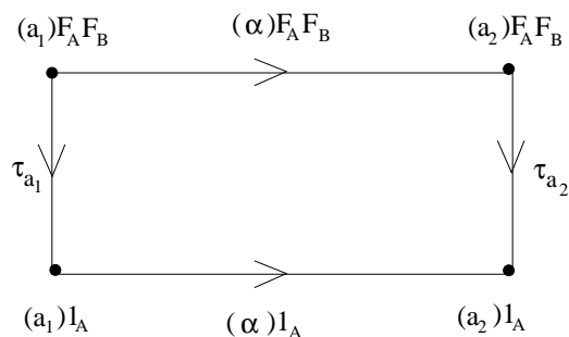
Figure 1.3.3: equivalent categories.
