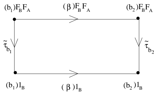
Figure 1.3.4: equivalent categories.
