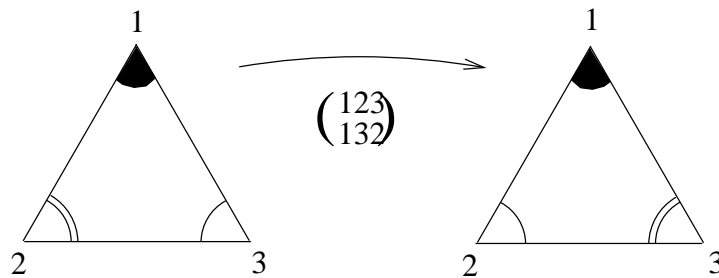
Figure 1.1.1: bijection.
