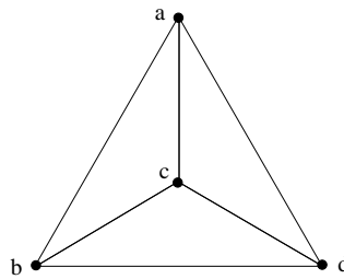
Figure 1.2.1: graph example.
